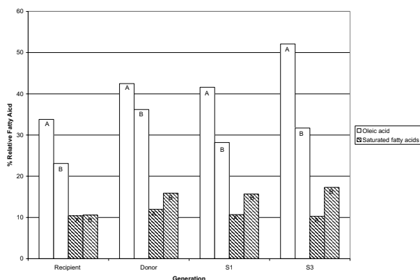
FIGURE 1 - Fatty acid comparison for two corn lines named High Oleic Acid (A) and High Total Saturated Fatty Acids (B).
